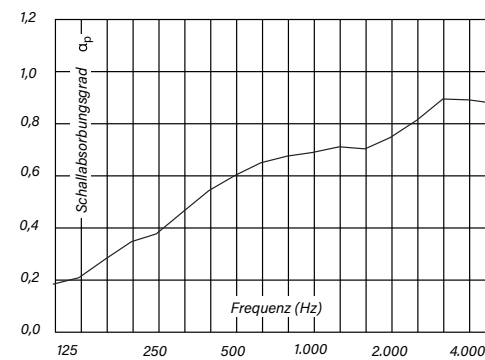
Sound absorption coefficient - Octave centre frequency
